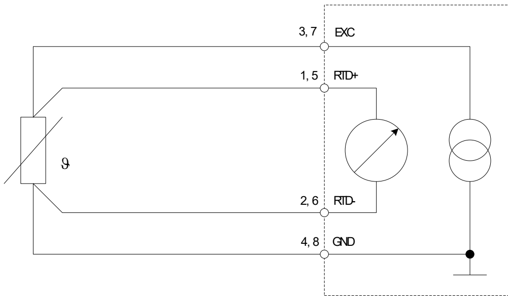
Fig. 4-4: Connection example: RTD sensors (4-wire circuit)
